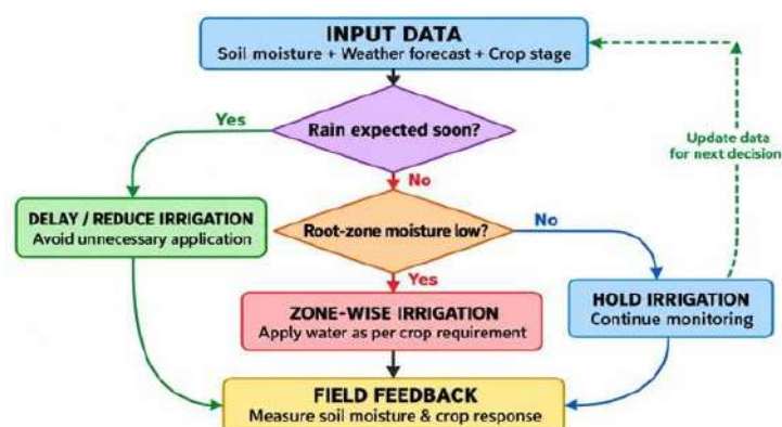
Fig. 2. Decision-tree pathway
